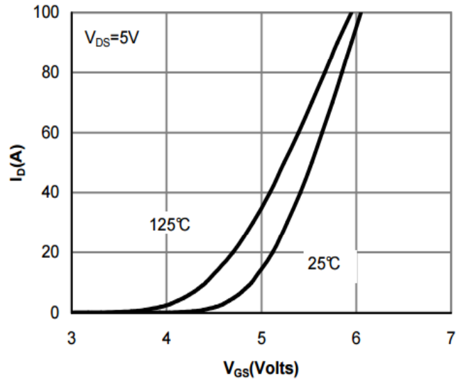
Transfer Characteristic
