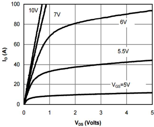
Output Characteristic
